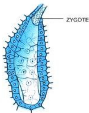
Figure 5: Helobial endosperm
