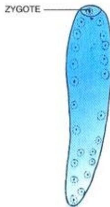
Figure 4: Cellular endosperm
