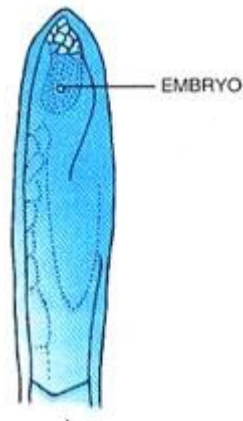
Figure 3: Nuclear endosperm
